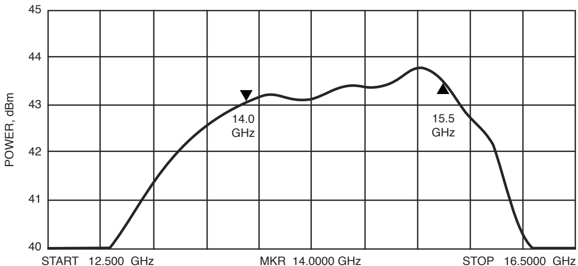
Figure 3. Psat vs Frequency
